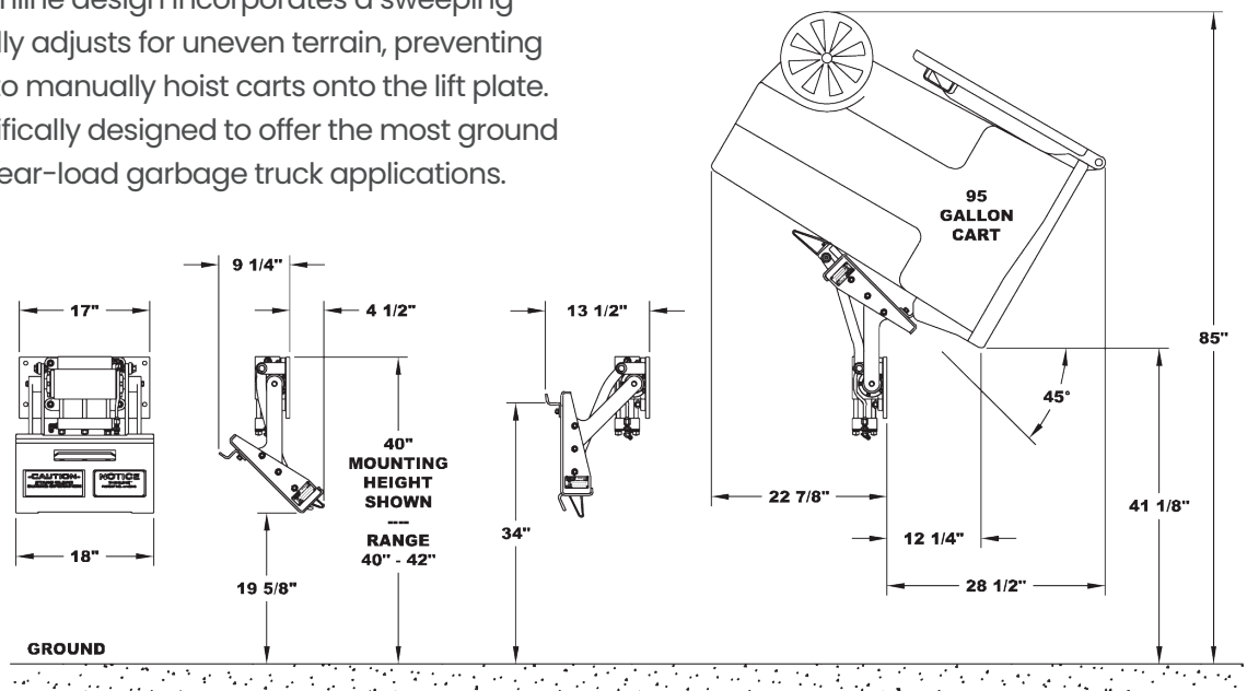
Patented Bayne Thinline Rack-and-Pinion Rotary Actuator
