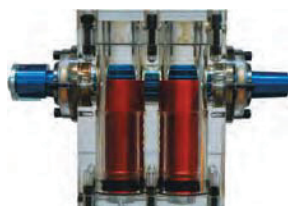
Patented Bayne Thinline Rack-and-Pinion Rotary Actuator
